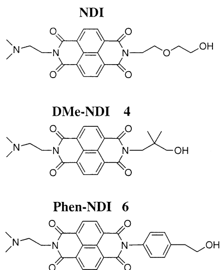
Figure 2. Structures of three naphthalene diimide based intercalators with linkers based upon 2-hydroxy-2-ethoxyethylamine (NDI), 3-hydroxy-2,2-dimethylpropylamine (DMe-NDI) and 2-hydroxy-2-phenylethylamine (Phen-NDI).
