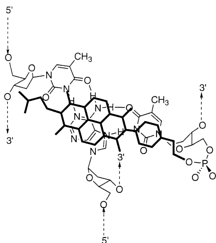
Figure 3. Possible relationship of the Phen-NDI intercalator (bold) and the terminal base triplet of a DNA triplex.
