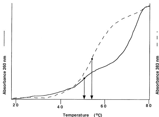
Figure 1. Thermally induced transitions for the DMe-NDI conjugate measured at 260 nm (solid line) and 383 nm (dashed line). The mid-points of the transitions (arrows) do not coincide suggesting a biphasic transition.
