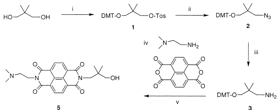
Scheme 1. (i) DMT-Cl, Tos-Cl, Py; (ii) \text{NaN}_3 , DMF, 90^\circ\text{C} ; (iii) \text{H}_2 Pd/C 10%, MeOH; (iv) isopropanol, \Delta ; (v) 3% trichloroacetic acid/ \text{CH}_2\text{Cl}_2 .
